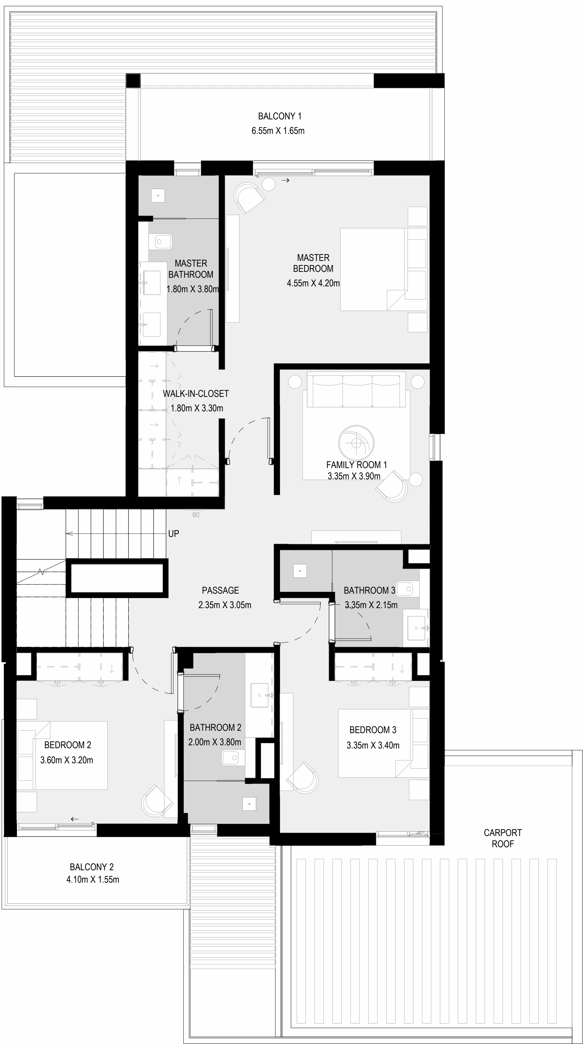
FIRST FLOOR
